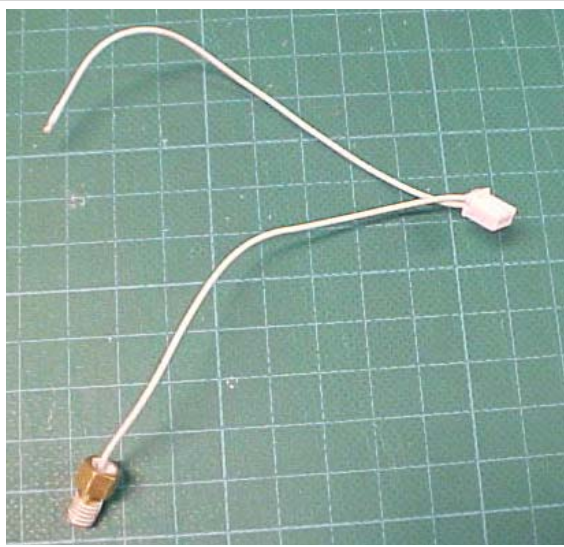
Part 290 - Thermister
