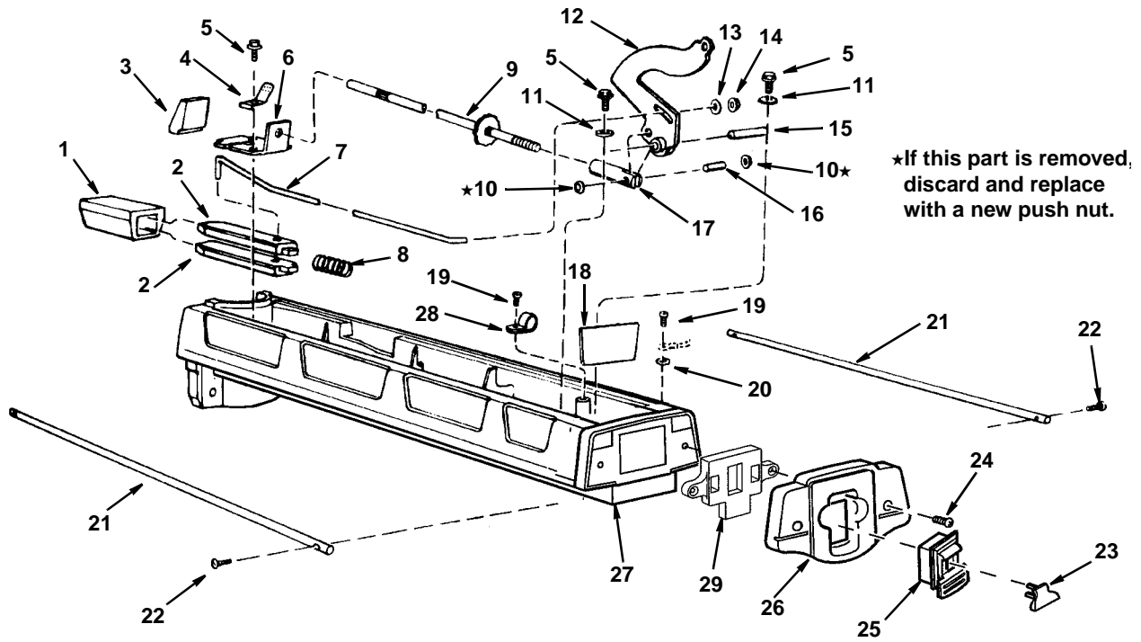
Figure 5 - Arm Assembly
